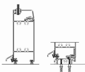
detalle umbral
